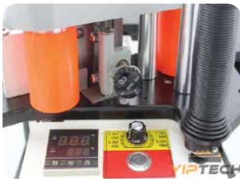
High-precision temperature control meter, real-time adjustment of hot melt temperature
